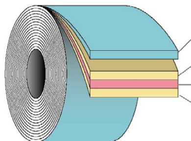
White paper coated with PE Side 2: Pure Acrylic adhesive Black PE foam 0.8 mm Side 1: Pure Acrylic adhesive
